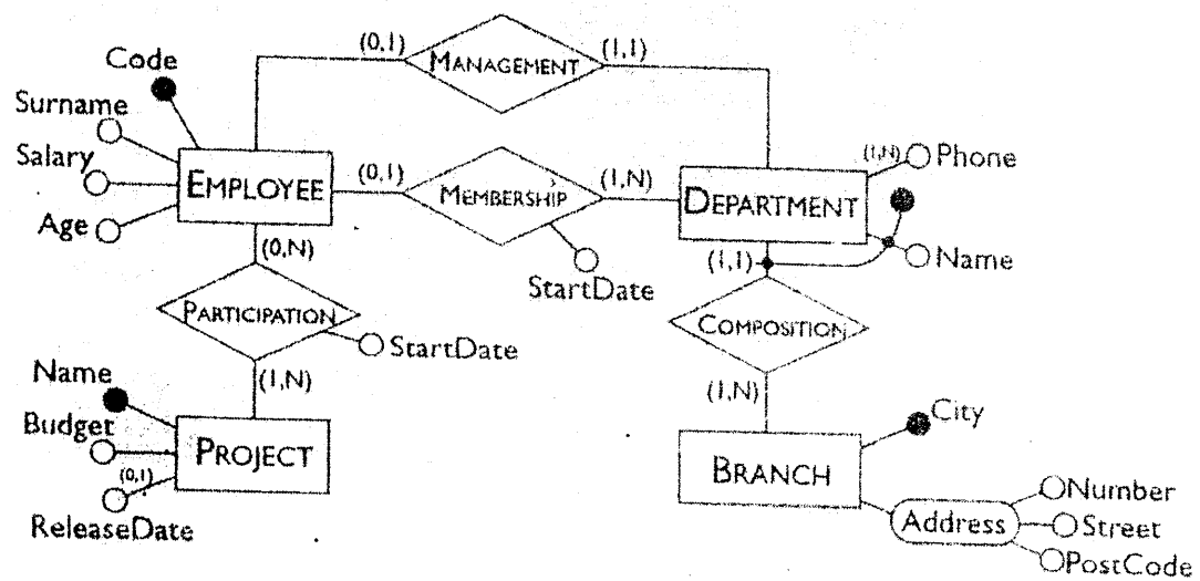
Fig.1 : An E-R schema on the personnel of a company
